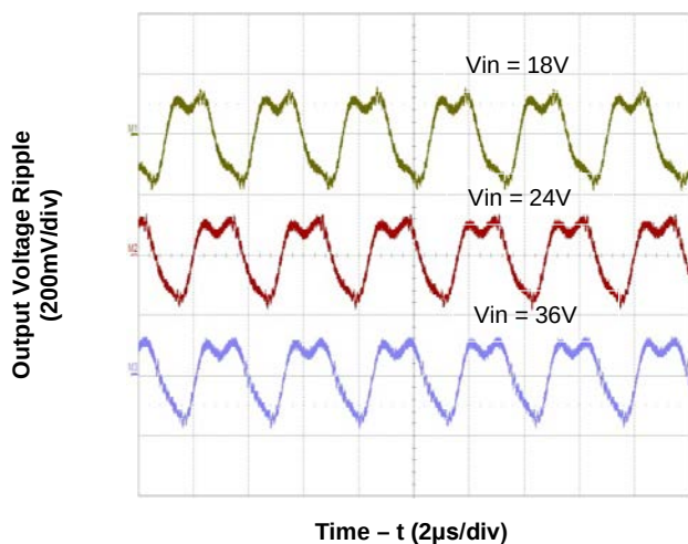
Figure 3. Output Voltage Ripple at Full Load (tested with 4x4.7µF ceramic output capacitors)
