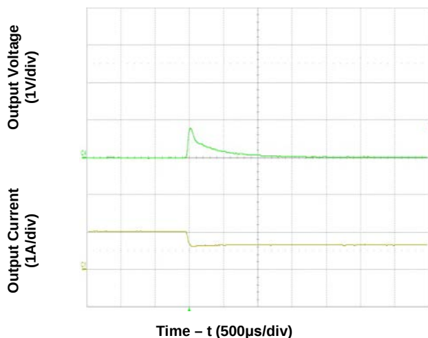
Figure 5. Transient Load Response (typical Vin, load current steps from 75% to 50% at a slew rate 0.1A/µs)
