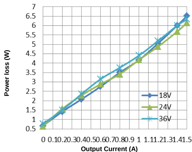
Figure 2. Power loss vs. Output Current (25°C)
