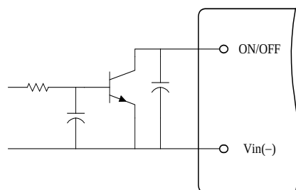
Figure 10. Opto Coupler Enable Circuit
