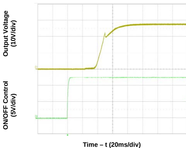
Figure 4. Start-Up from Enable Control (typical Vin, full load, no external output capacitor)
