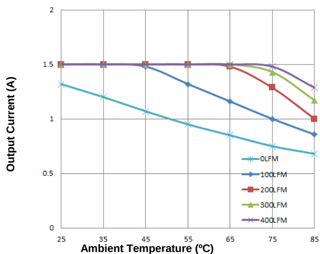
Figure 7. Current Derating Curve with Open Frame (Direction 3 (Ref. Figure 8); typical Vin, soldered interface)
