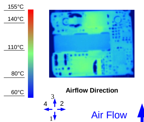
Figure 8. Thermal Image for Airflow Direction 3 (1.5A output, 55°C ambient, 200 LFM, typical Vin, open frame unit)
